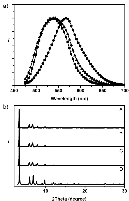
Figure 4. a) Emission spectra of freshly prepared 2 (■; \lambda_{\text{max}} = 538.8 nm), 2 soaked with Et_2O (●; \lambda_{\text{max}} = 567.0 nm), and 2 soaked with Et_2O and then MeOH (▲; \lambda_{\text{max}} = 540.0 nm) at \lambda_{\text{ex}} = 459.0 nm. b) PXRD of freshly prepared 2 (C), 2 soaked with Et_2O (B), 2 soaked with Et_2O and then MeOH (A), and the simulated pattern (D).
