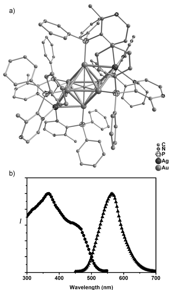
Figure 3. a) Molecular structure of the cationic part of [(C)(Au\text{-}mdppz)_6Ag_2](BF_4)_4 ( 3 ). b) Excitation (●) and emission (▲) spectra of 3 in the solid state; \lambda_{\text{max}}(\bullet) = 366.8 nm, \lambda_{\text{max}}(\blacktriangle) = 563.2 nm.
