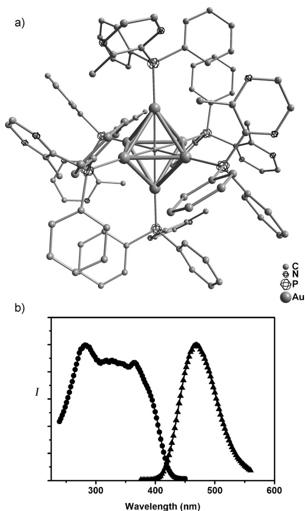
Figure 1. a) Molecular structure of the cluster linker [(C)(Au-mdppz)_6]-(BF_4)_2 ( 1 ) bearing six outward N donors. b) Excitation (●) and emission (▲) spectra of 1 in the solid state; \lambda_{max} (●) = 287.8 nm, \lambda_{max} (▲) = 468.4 nm.
